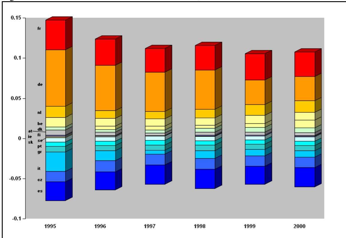
Figure 5. Trend of Theil Elements for 15 Countries, 1995-2000
