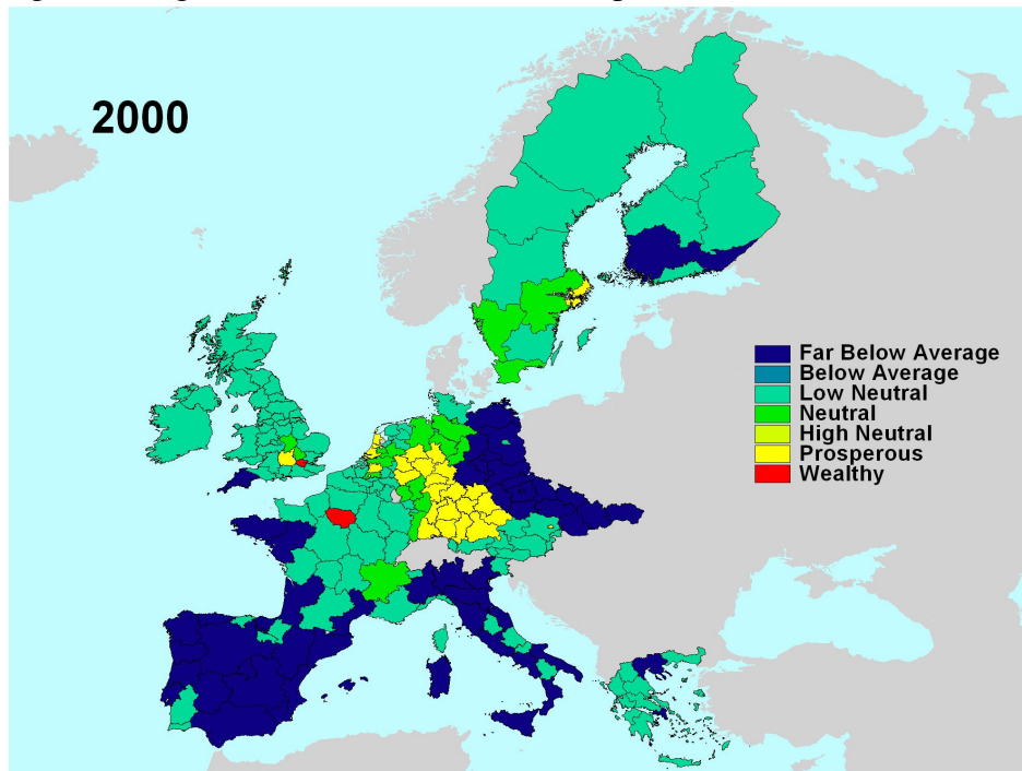
Figure 7. Regional Contribution to the European Theil for the Year 2000
