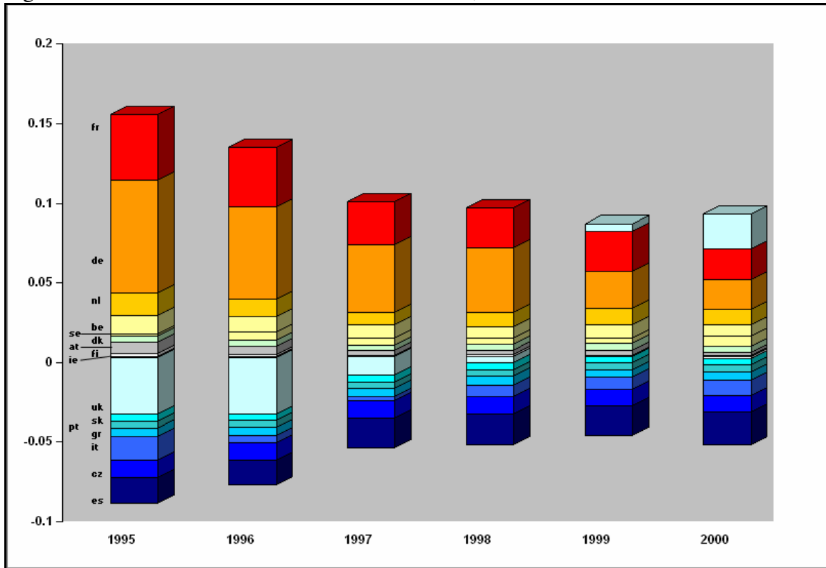
Figure 2. Trend of Theil Elements for 16 Countries, 1995-2000
