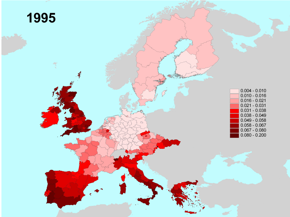
Figure 9. Within-Regions Between-Sectors Inequality, 1995
