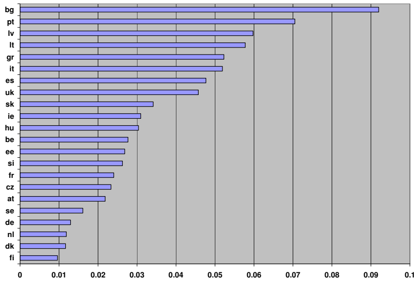
Figure 8. Theil's T Statistic Between Sectors, 1995-2000 Average Value
